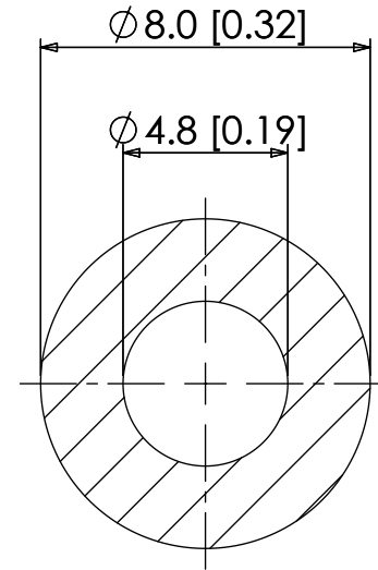
CROSS SECTION OF HOSE
